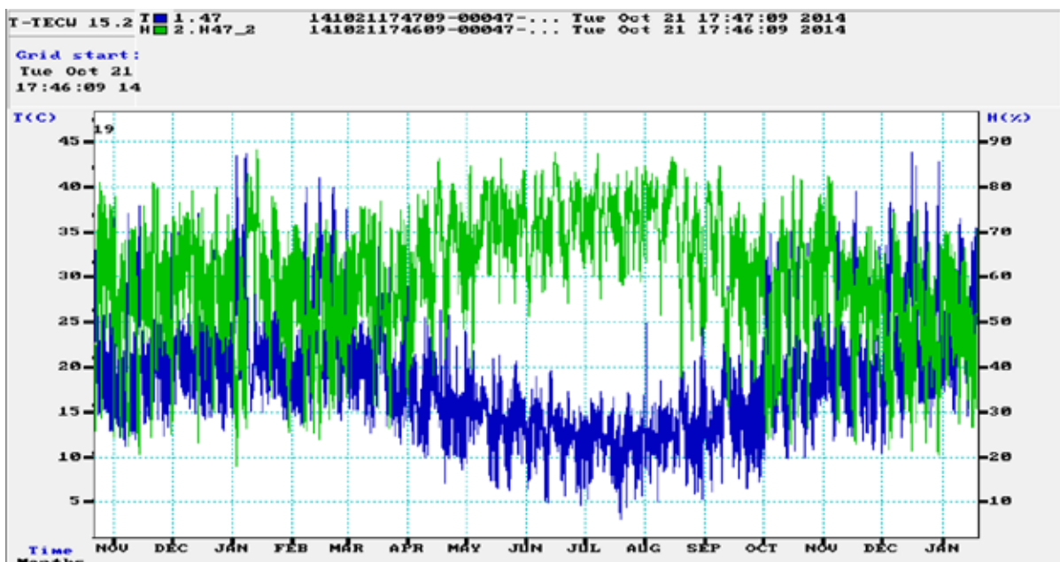
Outdoor temperature and humidity in Adelaide – from wireless T-TEC logger in wrap-around mode. This data set has 1.3 million logs, stored in the database.
